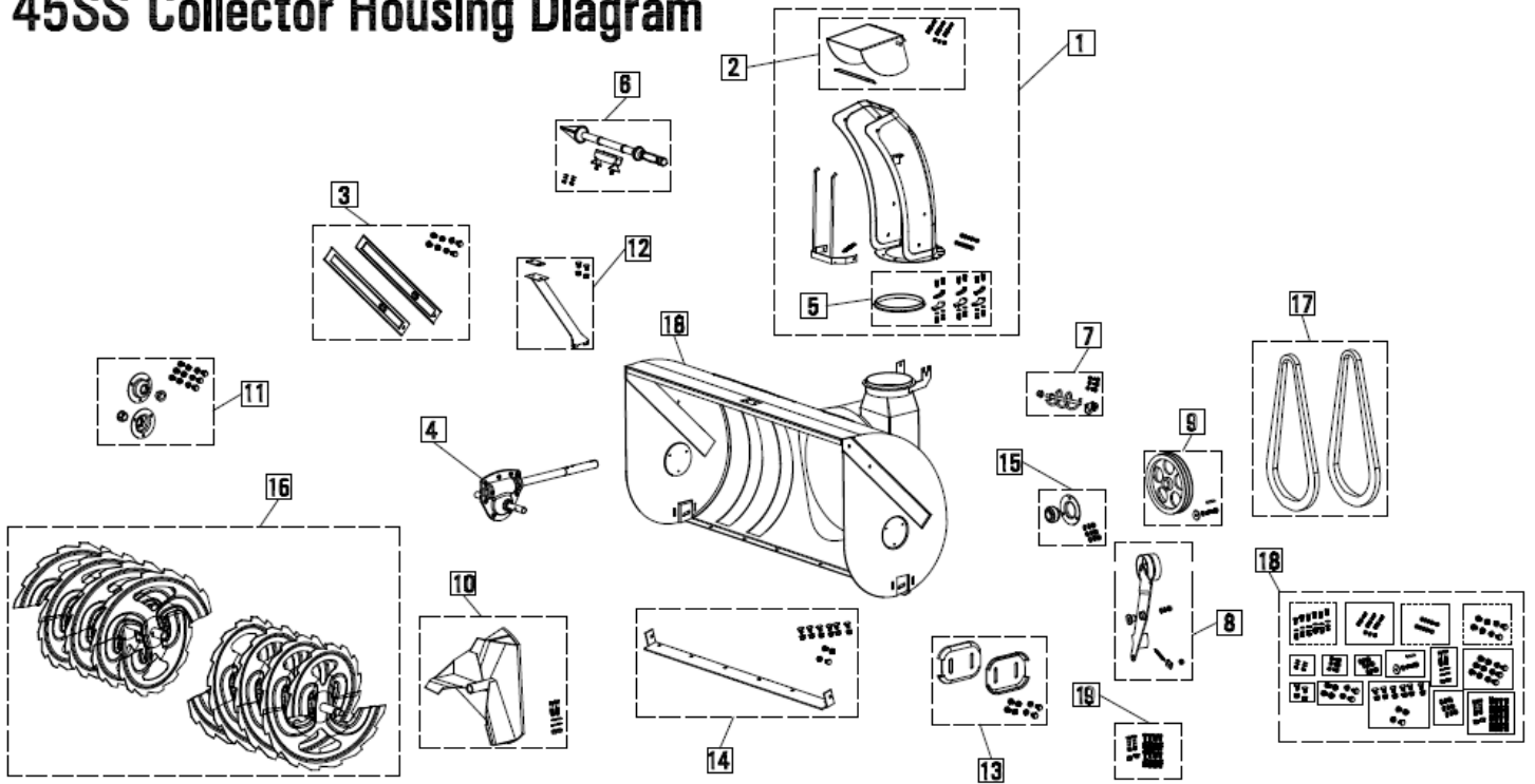
45SS Collector Assembly Diagram Key - Year Model 2012/13
