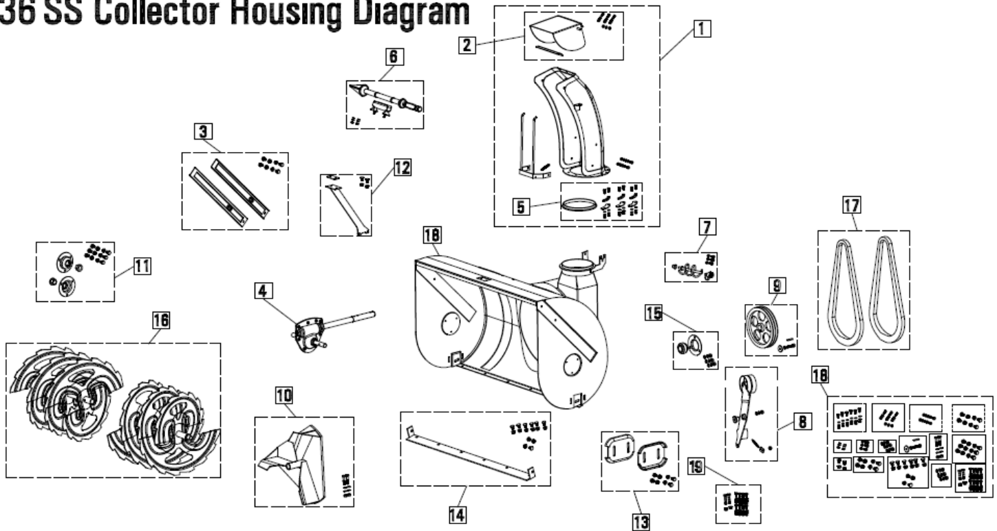
36SS Collector Assembly Diagram Key - Year Model 2012/13
