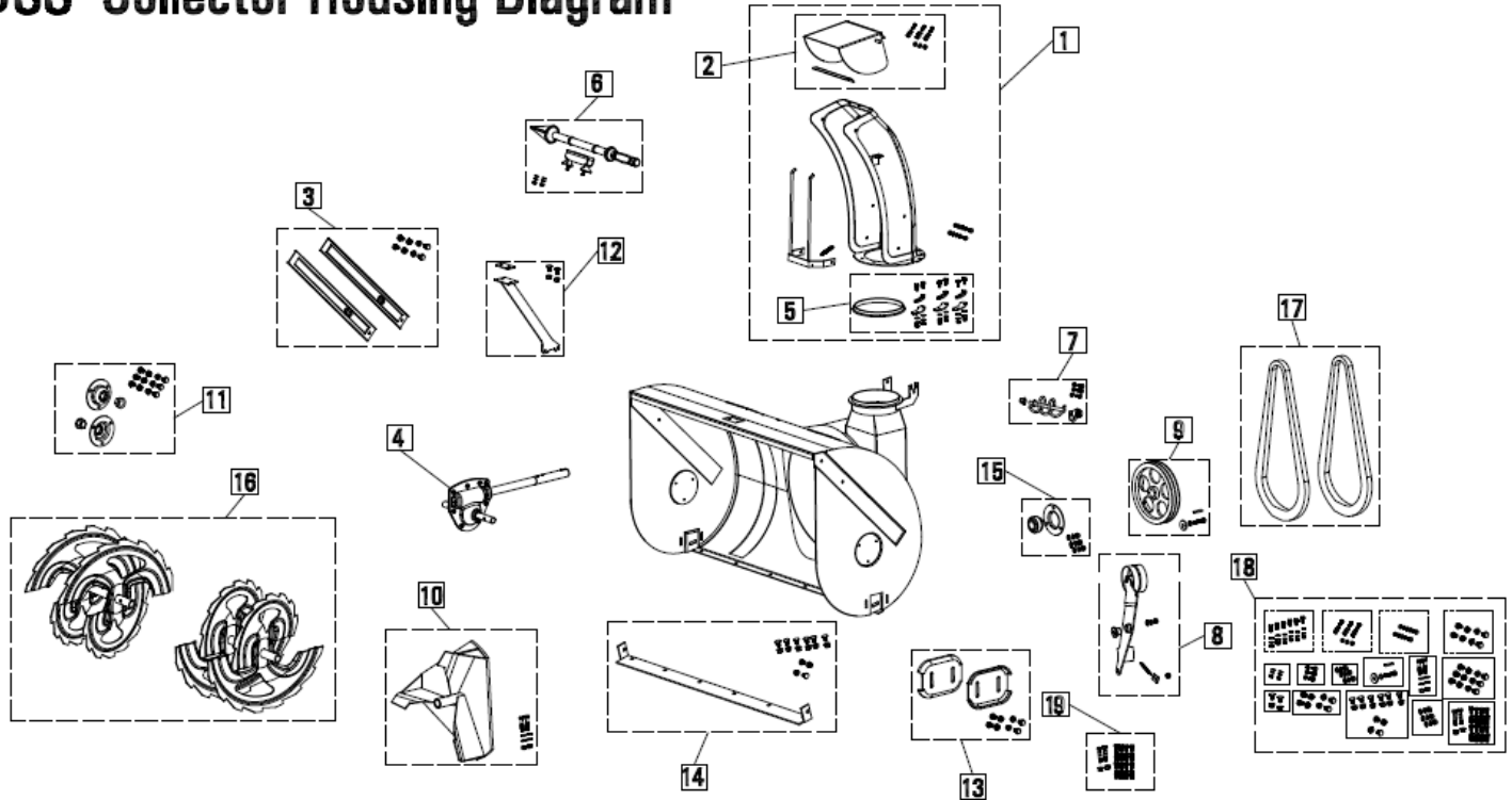
30SS Collector Assembly Diagram Key - Year Model 2012/13
